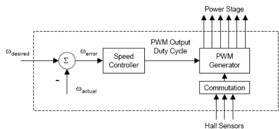
Fig. 2. Implementation of PID Speed Controller.
