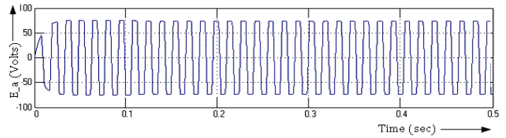
3(c) Back EMF Waveform for Phase-A.
