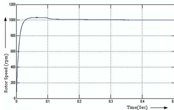
3(a) Rotor Speed vs. Time.
