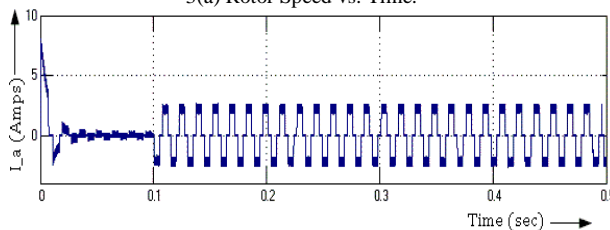
3(b) Phase Current Waveform for Phase-A.
